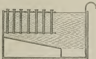
FIG. 2. BATH FOR HARDENING TAPS AND REAMERS.
